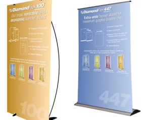
Multiple Models
